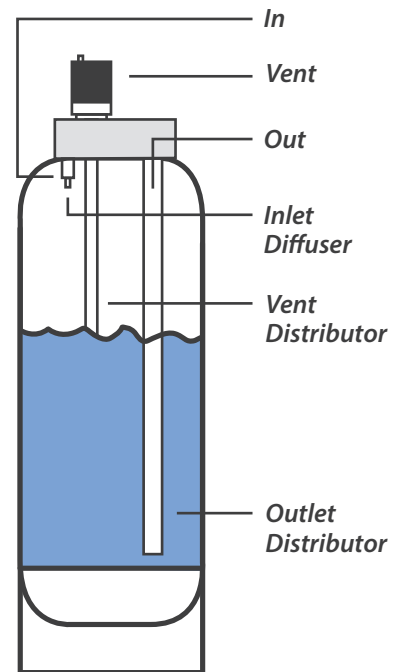
Large Aeration Tank
